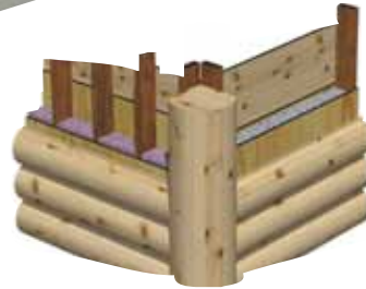
Panelized Home Corner Standard Insulation (left) & SIPs Panel (right)
